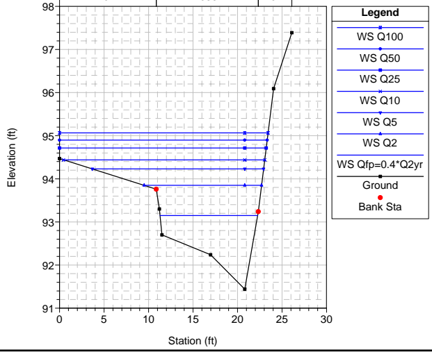
534 Plan: 10-Mile Existing 9/27/2006 RS = 1
