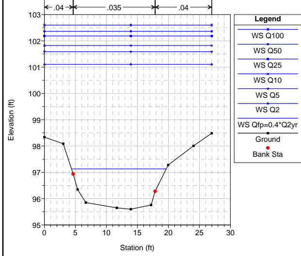
534 Plan: 10-Mile Existing 9/27/2006 RS = 5 Culv
