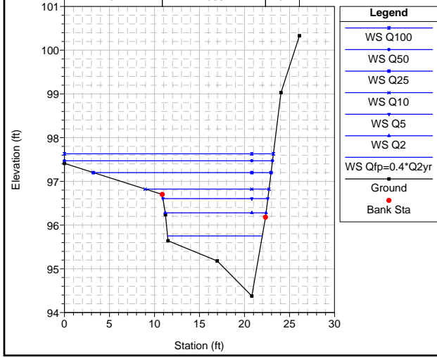
534 Plan: 10-Mile Existing 9/27/2006 RS = 2
