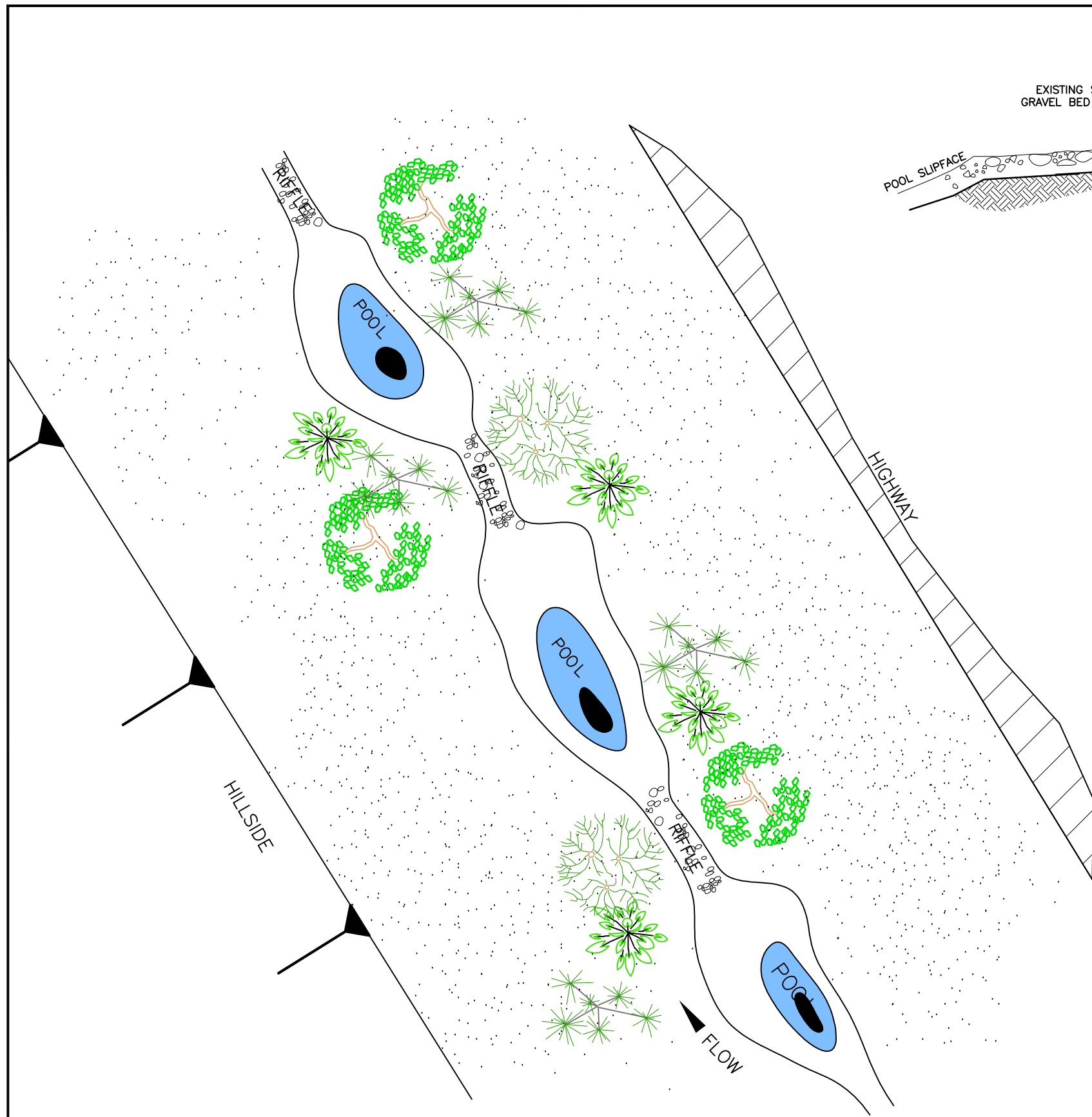
PLAN VIEW POOL-RIFFLE NOT TO SCALE
